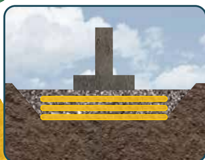
Foundation cushioning, soil stabilisation
