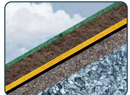
Stabilisation of landfill slopes
